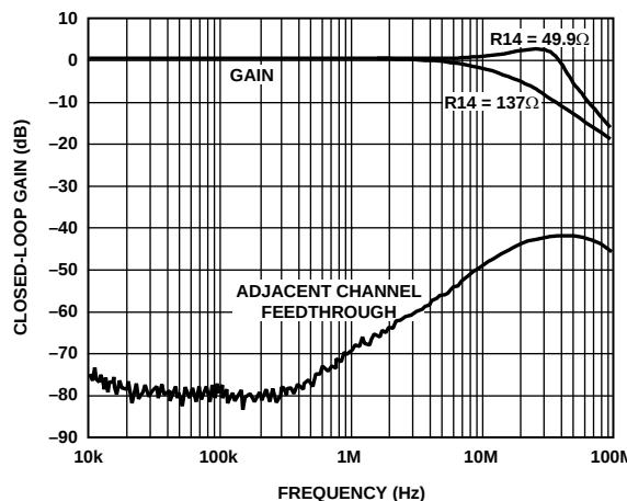
Figure 48. A Plot of the AC Response of the Video Keyer
